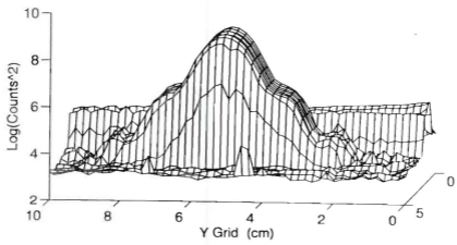
Figure 4.13 3 D representation of the monostatic acoustic pulse for 1.3 MHz and wire of radius 50 microns in log and linear space.
